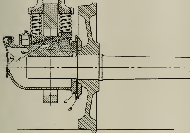
AXLE BOX FOR GUIDING WHEEL OF END TRUCK.
